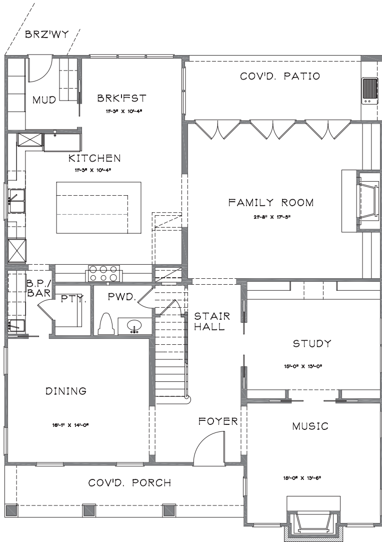
First Floor
